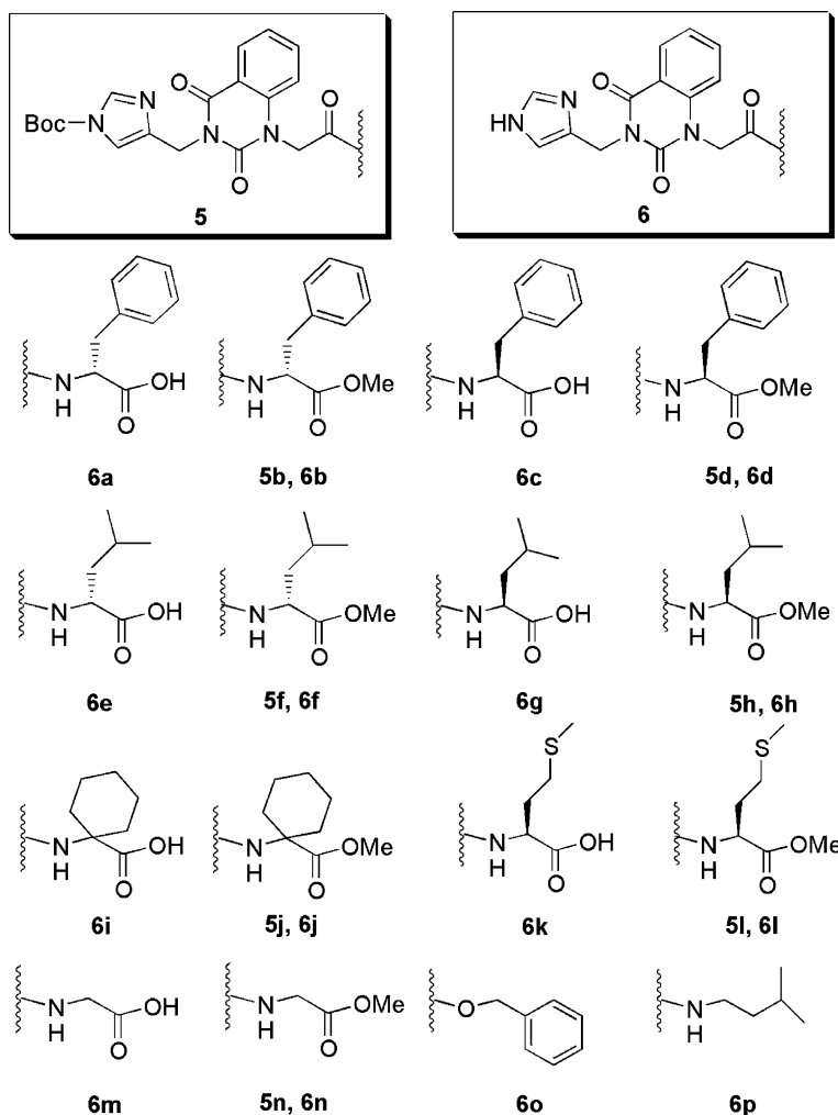
Figure 4. Benzoyleneurea-based PGGTase-I inhibitors.
