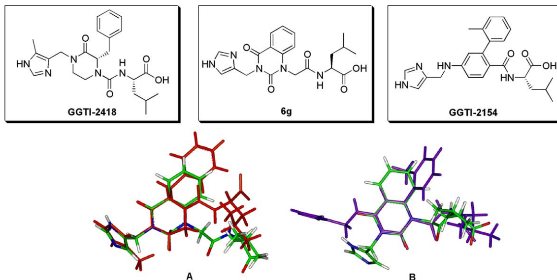
Figure 2. Comparison of proposed novel PGGTase-I inhibitor 6g (atom color) with (a) GGTI-2418 (orange) and (b) GGTI-2154 (purple). Inhibitors were built and minimized in the Insight II (2000) suite of programs builder module.
