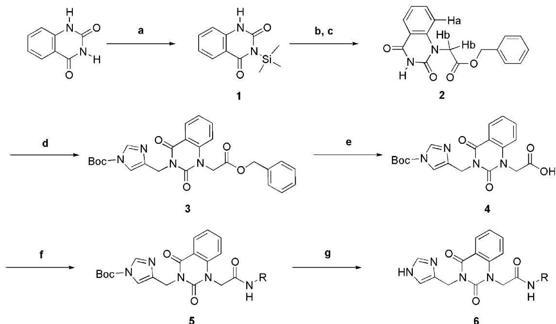
Scheme 1. Reagents and conditions: (a) (CH_3)_3SiNHSi(CH_3)_3 , (NH_4)_2SO_4 , toluene; (b) benzyl chloroacetate, KI, toluene; (c) EtOH, 90% for three steps; (d) 1- t -butoxycarbonyl-4-chloromethylimidazole, K_2CO_3 , acetone, 89%; (e) H_2 , Pd/C, MeOH, CH_2Cl_2 , 91%; (f) H_2NR , HOBT, EDCI, Et_3N , DMF, 25–100%; (g) TFA, 82–100% or NaOH, 81–100%.
