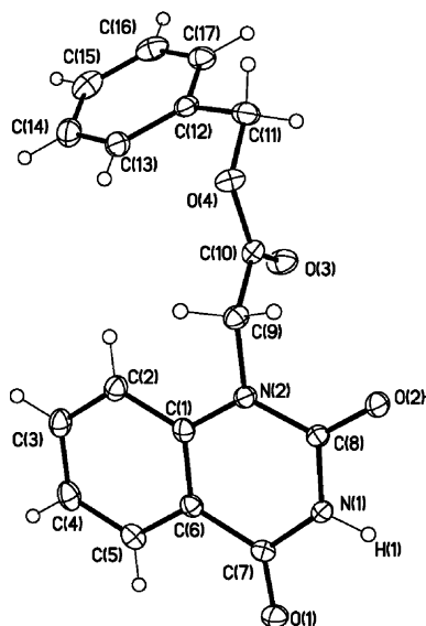
Figure 3. X-ray crystal structure of compound 2.
