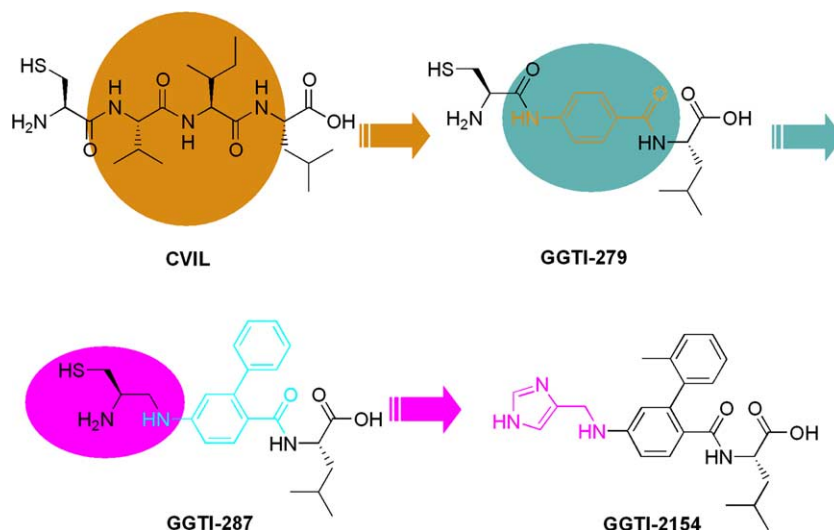
Figure 1. Evolution of CAAX peptidomimetic PGGTase-I inhibitor design.
