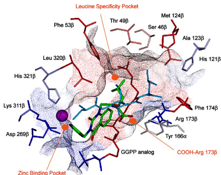
Figure 5. Comparison of the GOLD-predicted docked conformation of 6g (atom color) in the active site of PGGTase-I (pdb 1N4Q, colored by hydrophobicity, red hydrophobic to blue hydrophilic) with the enzyme bound conformation of the native substrate peptide CVIL (cyan blue).
